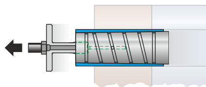
Disassemble GripCon
