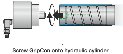
Screw GripCon onto hydraulic cylinder
