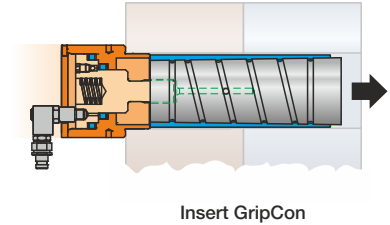
Insert GripCon
